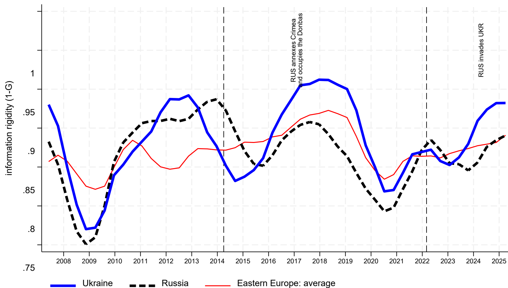
Figure 14. Information rigidity.
